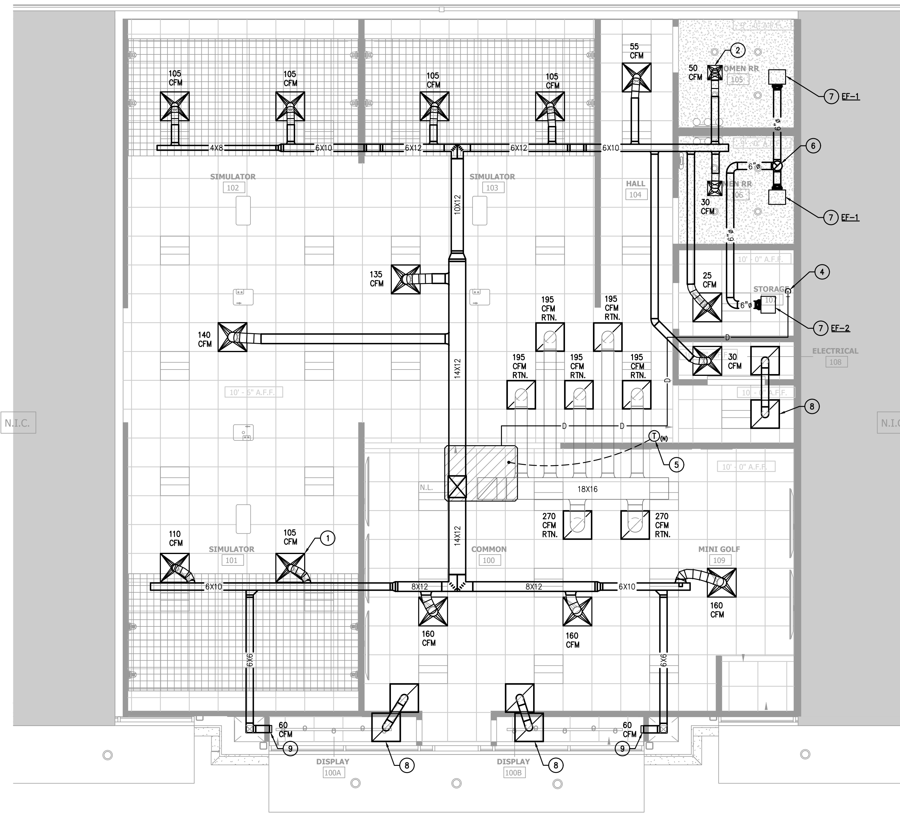
01 MECHANICAL PLAN SCALE: 1/8"=1'-0"
