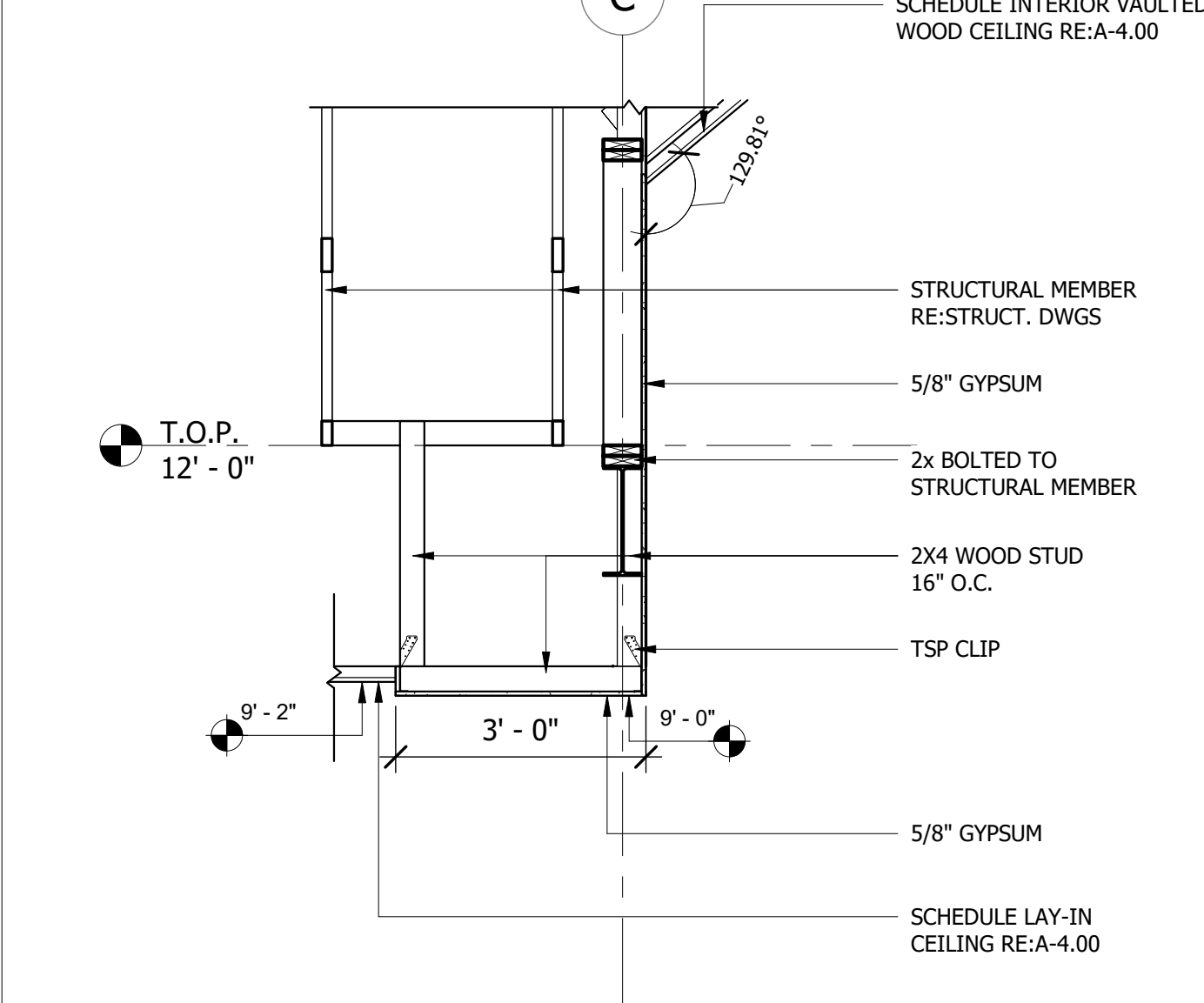
3 CORRIDOR FURR-DOWN 1/2" = 1'-0"
