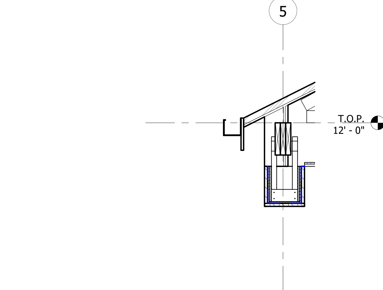
5 Detail 5 1/2" = 1'-0"
